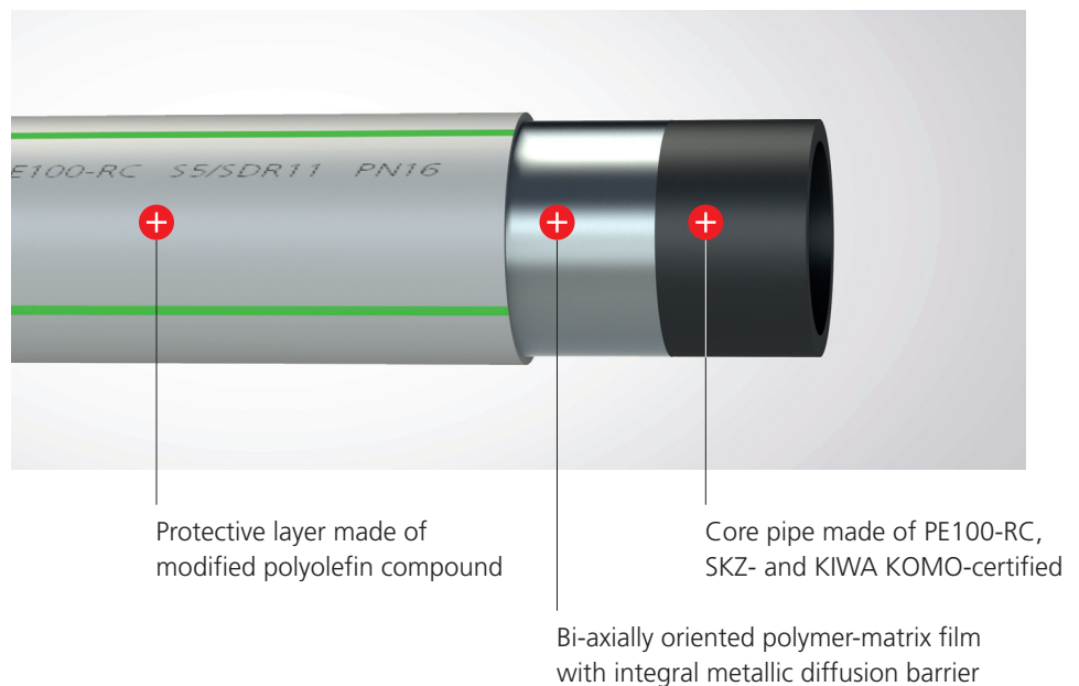
2 Pipe construction
